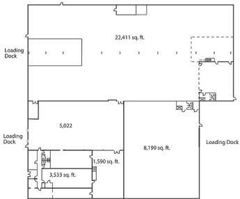
MAIN LEVEL Scale: 3/64" = 1'-0"
